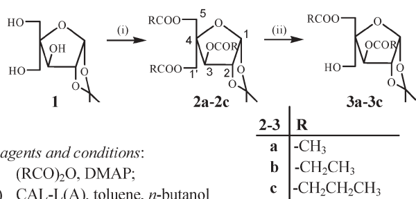
Scheme 1 Lipase-catalyzed selective deacylation studies on triacylated pentofuranoses 2a–2c .
